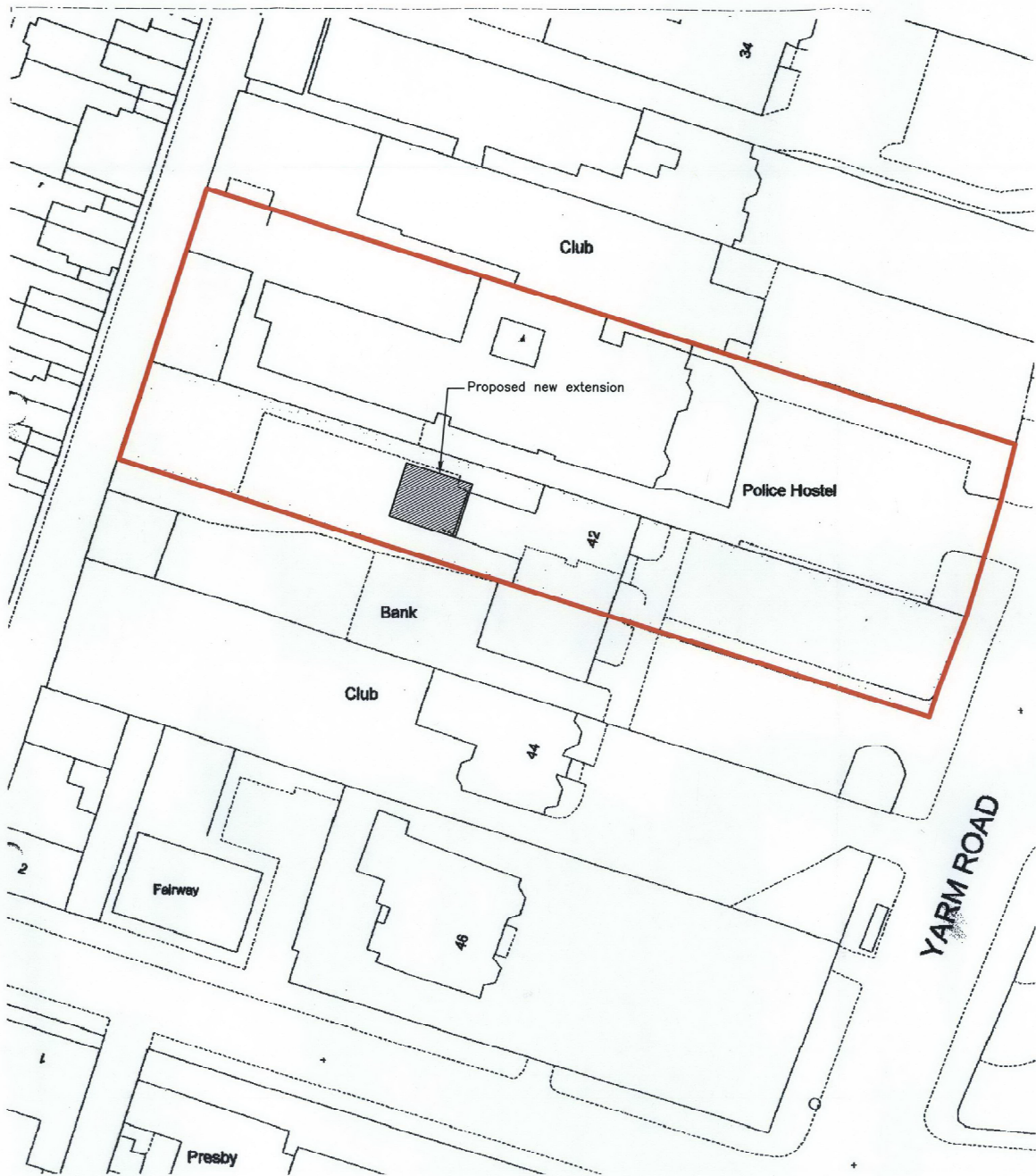
Site Plan Scale: 1/500 40/42 Yarm Road
